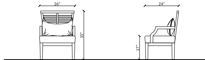
SINGLE SEATER FRONT VIEW
